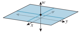
Figure 10.11: The w = 1 plane in xyw -space.
