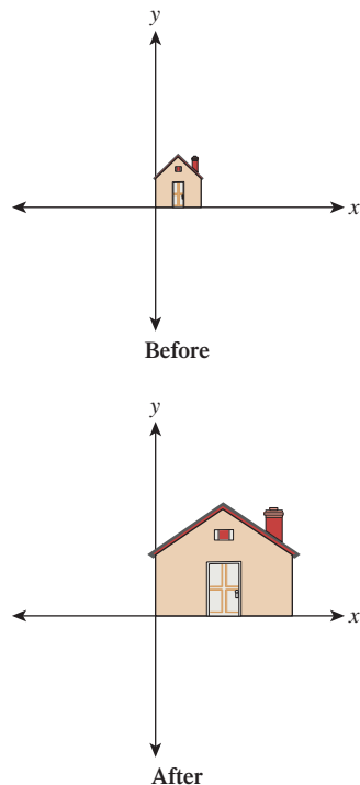
Figure 10.2: T_2 stretches the x -axis by three and the y -axis by two.
