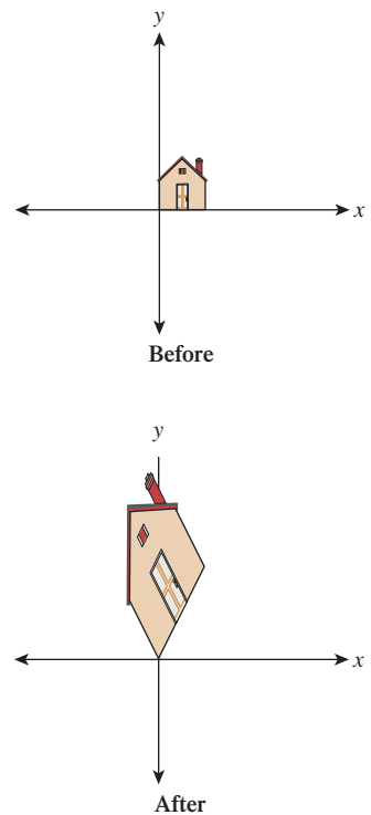
Figure 10.4: A general transformation. The house has been quite distorted, in a way that's hard to describe simply, as we've done for the earlier examples.
