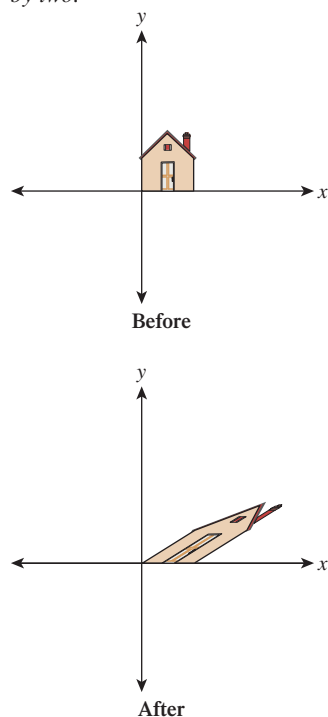
Figure 10.3: A shearing transformation, T_3 .
